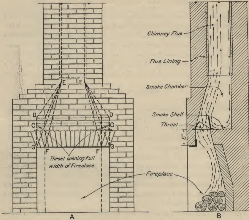
FIG. 13.—A. Top of throat damper is at DD, smoke shelf at CC. Side wall should not be drawn in until the height DD is passed. This assures full area. If the drawing is done as indicated by lines EF and EG, the width of the throat becomes less than the width of the opening and causes the air currents to pile up in the corners of the throat, resulting frequently in a smoky fireplace. B. Correct fireplace construction.
