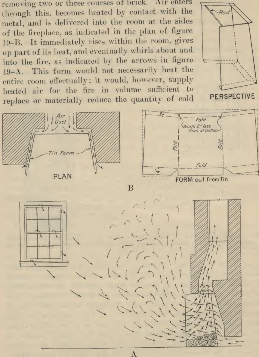
FIG. 19.—Simple form of warm-air flue for outside chimney. Air required for feeding the fire is brought in from the outside around a metal form set in the fireplace, with a space between it and the back and sides of the brickwork. As the cold outside air passes around the metal it becomes heated and is delivered into the room at a temperature much higher than where it is pulled in through window and door cracks. The result is a much more comfortable room.
