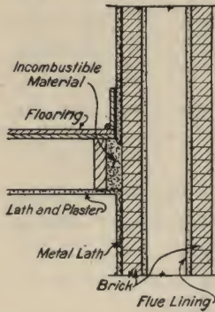
FIG. 10.—No woodwork should be permitted closer than 2 inches to the outside face of a chimney. Baseboards in front of chimneys should be protected with asbestos board.
