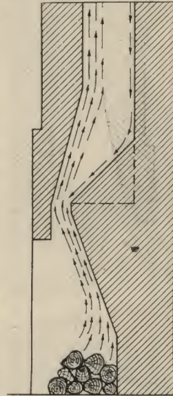
FIG. 16.—This construction without a throat damper directs the down draft so that it meets the up draft almost at the throat, which is more faulty than the construction shown in fig. 15, for there the lid of the damper deflects the down current.
