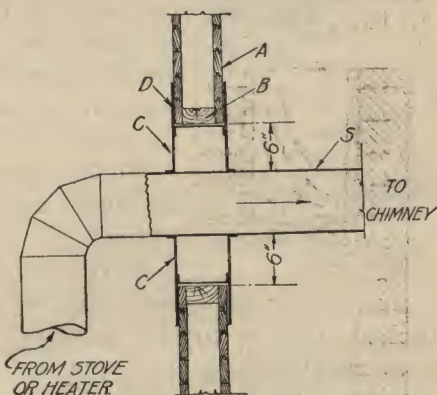
FIG. 9.—Smoke pipe passing through a partition. A, \frac{3}{4} -inch sides of partition; B, 2 by 4 studs in partition; C, ventilating holes in the double galvanized iron ventilating thimble D. Thimble should be at least 12 inches larger than pipe S.
